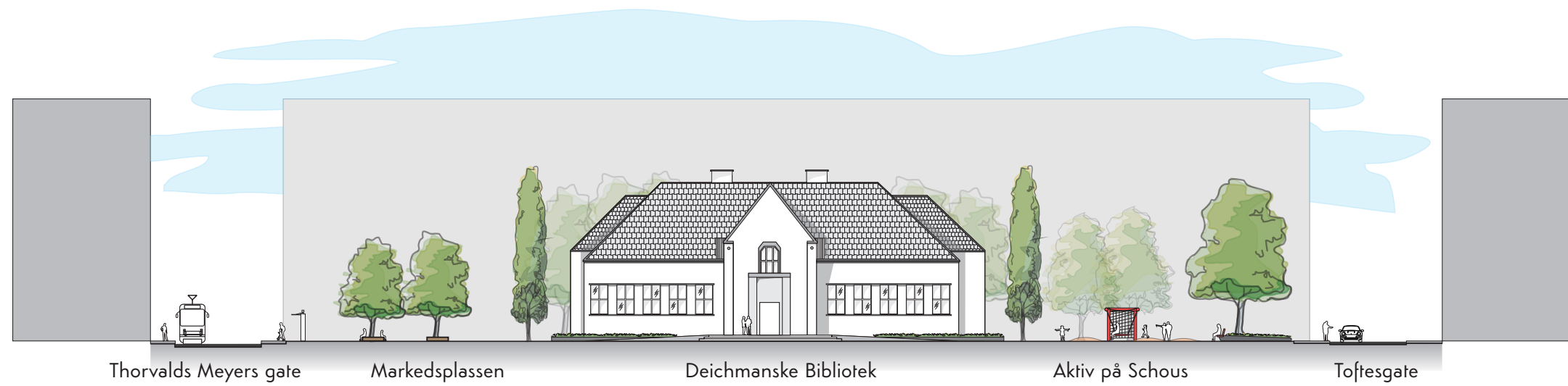
SNITT A - A' Thorvalds Meyers gate - Toftesgate
